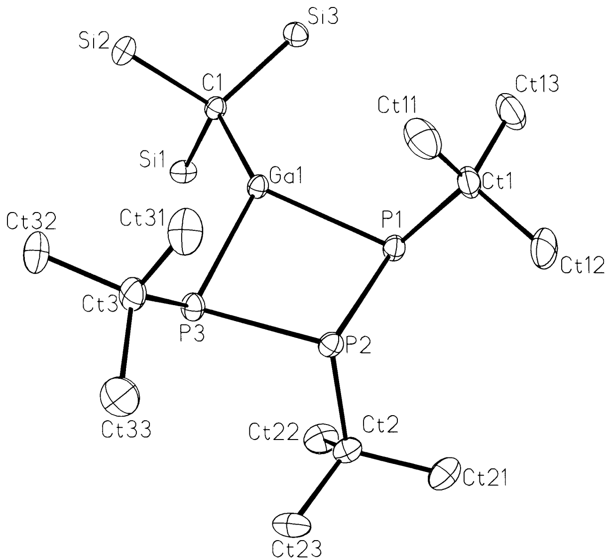
Fig. 1 Molecular structure of compound 2 . Only one of the two independent molecules is shown; a similar numbering scheme holds for the second molecule. Thermal ellipsoids are drawn at the 40% probability level. Methyl groups of the \text{C}(\text{SiMe}_3)_3 substituent and hydrogen atoms are omitted. Important bond lengths (pm) and angles ( ^\circ ): Ga1–C1 200.4(2), Ga1–P1 235.77(7), Ga1–P3 237.00(7), P1–P2 221.72(9), P2–P3 221.73(9), Ga2–C2 199.9(2), Ga2–P4 236.22(7), Ga2–P6 235.02(6), P4–P5 221.85(9) and P5–P6 221.69(9); Ga1–P1–P2 84.91(3), P1–P2–P3 98.12(3), P2–P3–Ga1 84.62(3), P1–Ga1–P3 90.23(2), Ga2–P4–P5 84.47(3), P4–P5–P6 98.15(3), P5–P6–Ga2 84.78(3) and P4–Ga2–P6 90.66(2).
